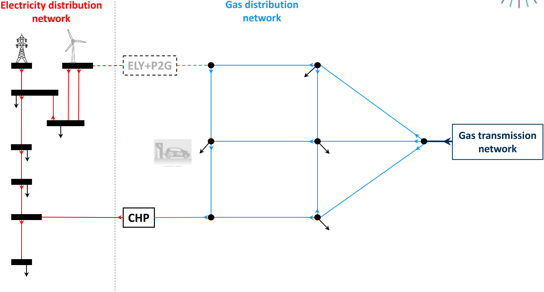
Distribution networks: Base Case
